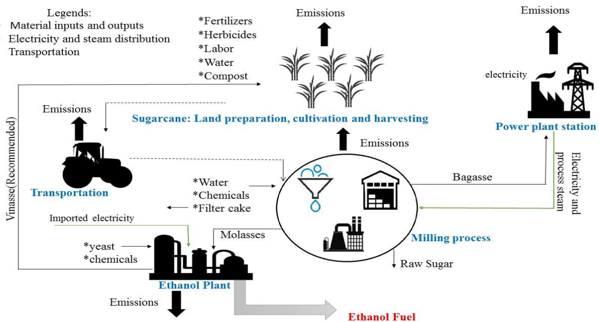
Figure 1. System boundary of molasses-based ethanol production.
